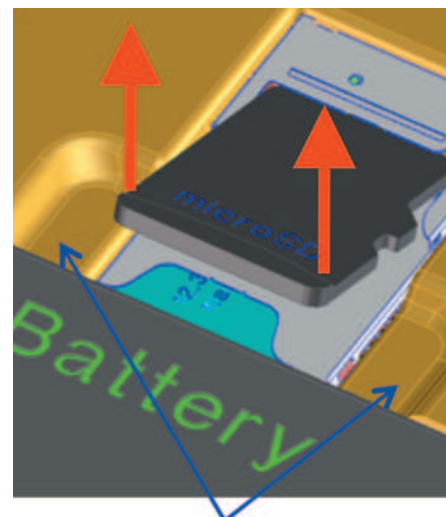
Recommended Shape (Easy to eject a microSD card)
