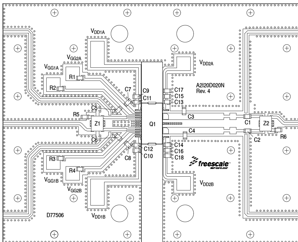
Figure 3. A2I20D020NR1 Test Circuit Component Layout
