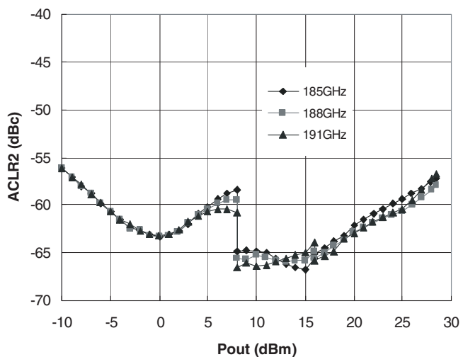
Figure 5. Adjacent Channel Leakage Ratio 2 vs. Output Power
