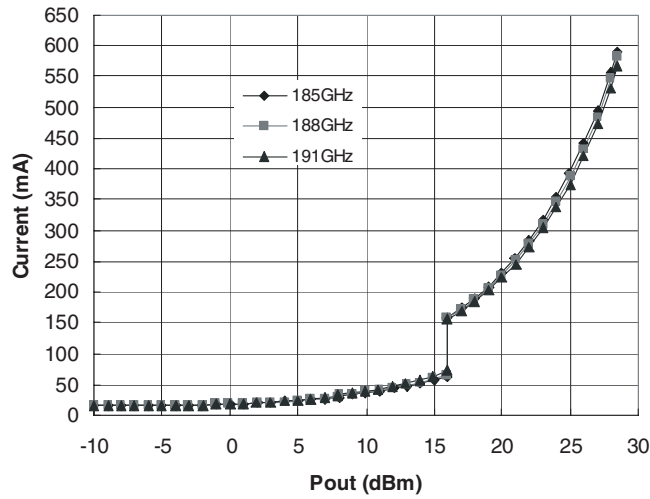
Figure 6. Total Current vs. Output Power
