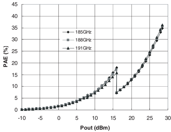
Figure 8. Power Added Efficiency vs. Output Power
