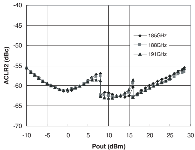
Figure 10. Adjacent Channel Leakage Ratio 2 vs. Output Power
