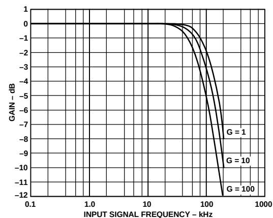
Figure 5. Normalized Gain as a Function of Signal Frequency
