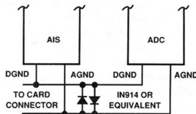
Figure 11. Ground-Fault Protection Diodes
