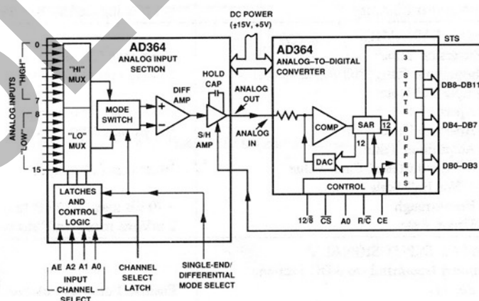
AD364 FUNCTIONAL BLOCK DIAGRAM
