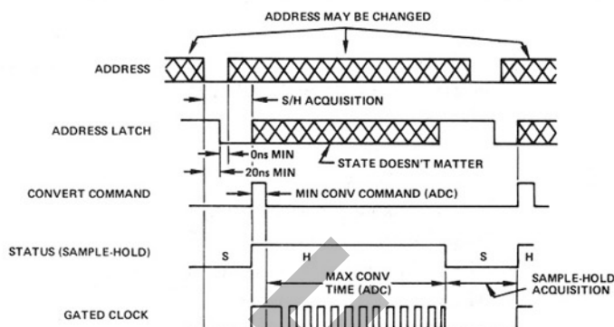
Figure 3. AD363 Timing Diagram
