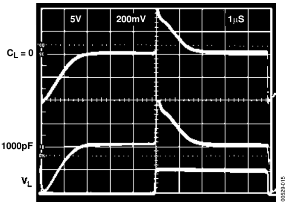
Figure 16. Output Response with Capacitive Load
