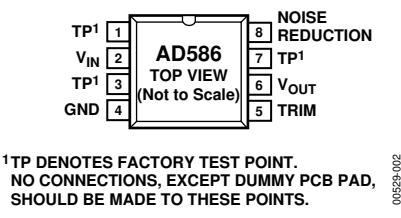
Figure 2. Pin Configuration (N-8)
