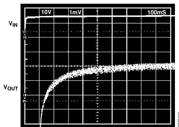
Figure 11. Turn-On with 1 \mu\text{F} C_N Characteristics
