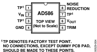
Figure 4. Pin Configuration (R-8)
