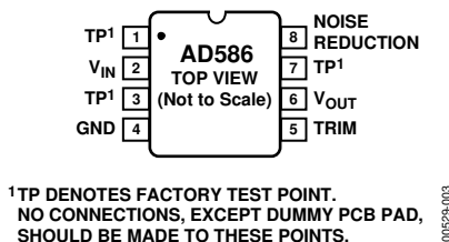
Figure 3. Pin Configuration (Q-8)
