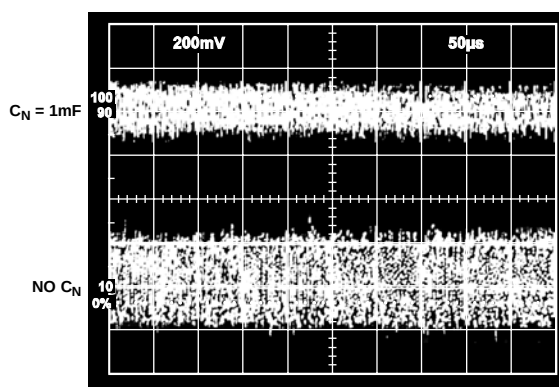
Figure 8. Effect of 1\text{ }\mu\text{F} Noise Reduction Capacitor on Broadband Noise
