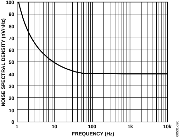
Figure 20. Input Noise Voltage Spectral Density
