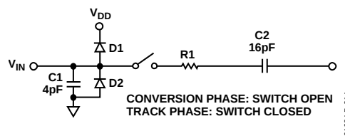
Figure 14. Equivalent Analog Input Circuit
