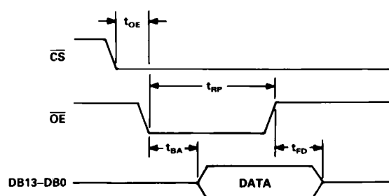
Figure 3. EOC Timing
