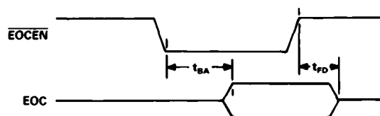
Figure 2. Output Timing
