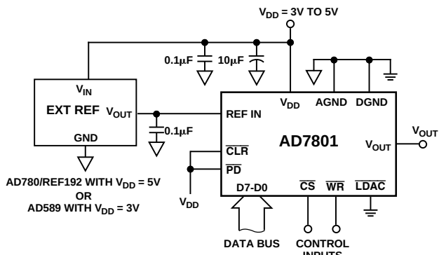
Figure 28. Typical Configuration Using An External Reference
