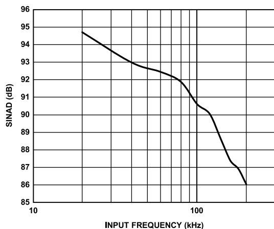
Figure 18. SINAD vs. Input Frequency
