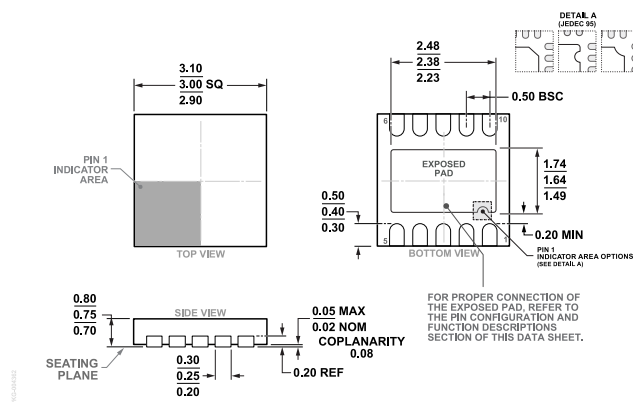
Figure 51. 10-Lead Lead Frame Chip Scale Package [LFCSP] 3 mm × 3 mm Body and 0.75 mm Package Height (CP-10-9) Dimensions shown in millimeters
