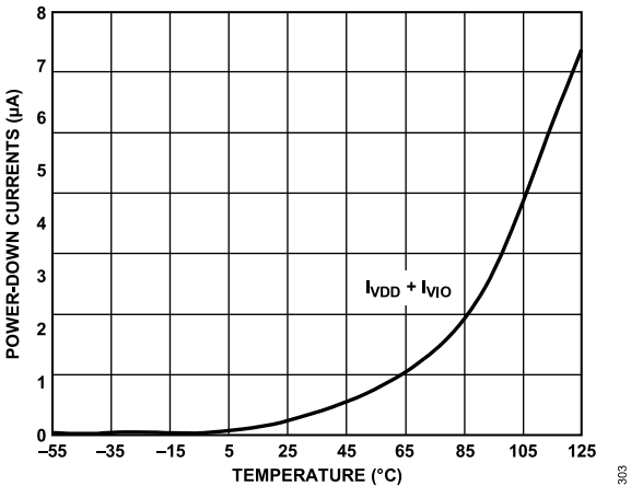
Figure 25. Power-Down Currents vs. Temperature
