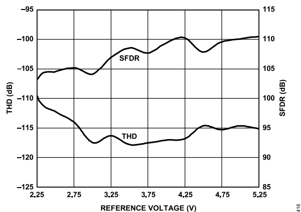
Figure 19. THD and SFDR vs. Reference Voltage
