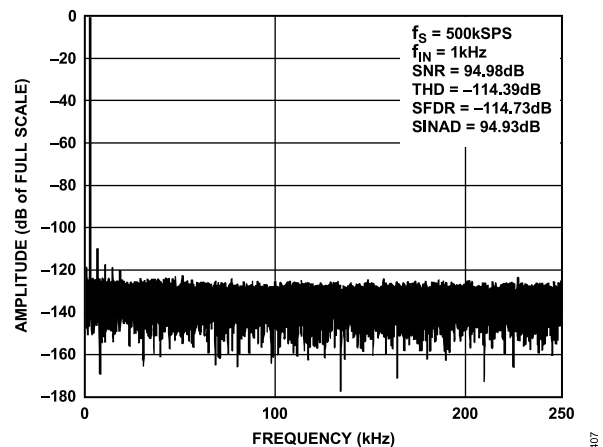
Figure 6. AD7916 FFT Plot, REF = 5 V
