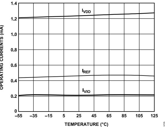
Figure 26. Operating Currents vs. Temperature (AD7915)
