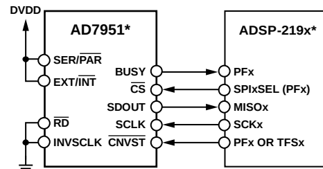
Figure 46. Interfacing the AD7951 to SPI Interface
