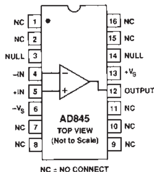
16-Lead SOIC (R-16) Package
