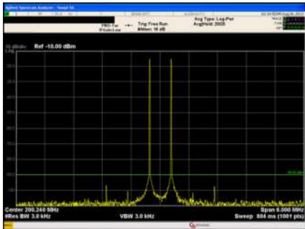
Figure 15. Two-Tone Third IMD Performance, f_c = 200 MHz, f_{DAC} = 1228.8 MHz, -9 dBFS
