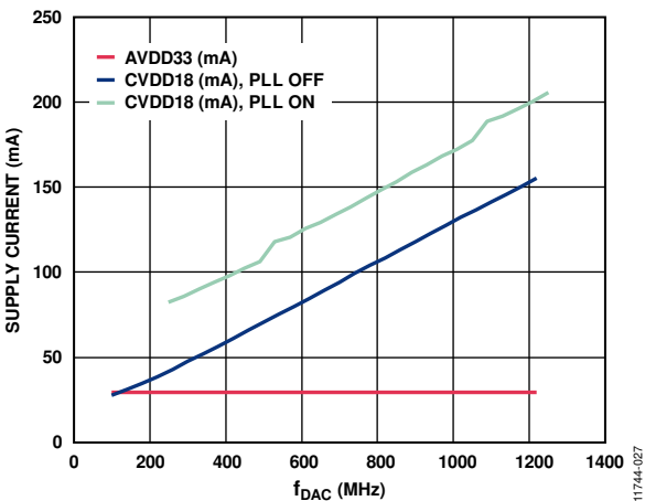
Figure 22. CVDD18 and AVDD18 Current vs. f_{DAC}
