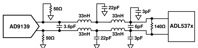
Figure 50. DAC Modulator Interface with Fifth-Order, Low-Pass Filter
