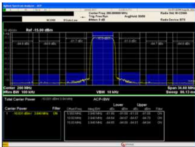
Figure 16. 1-Carrier WCDMA ACLR Performance, f_c = 200 MHz, f_{DAC} = 1228.8 MHz
