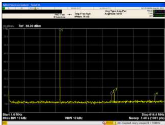
Figure 17. Single-Tone Performance, f_c = 200 MHz, f_{DAC} = 1228.8 MHz
