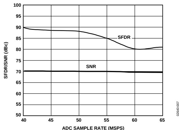
Figure 8. AD9238-65 Single-Tone SNR/SFDR vs. FS with f_{IN} = 32.5 MHz
