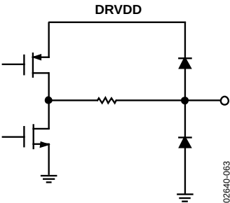
Figure 30. Equivalent Digital Output Circuit
