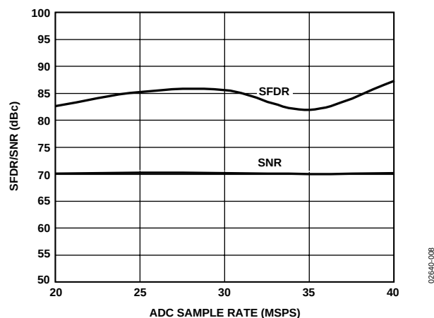
Figure 9. AD9238-40 Single-Tone SNR/SFDR vs. FS with f_{IN} = 20 MHz
