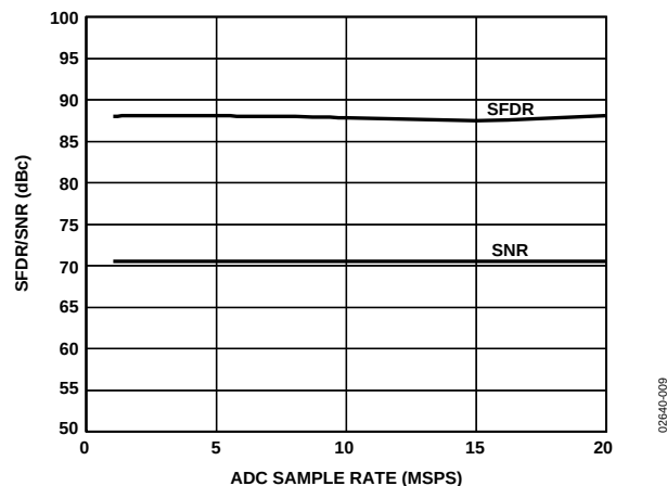
Figure 10. AD9238-20 Single-Tone SNR/SFDR vs. FS with f_{IN} = 10 MHz
