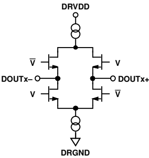
Figure 29. Equivalent Digital Output Circuit
