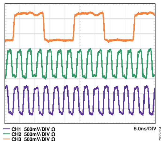
Figure 64. LVDS Output Timing Example in ANSI-644 Mode (Default)
