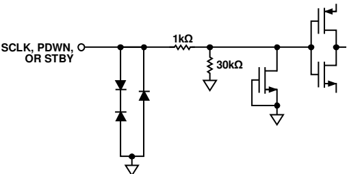
Figure 30. Equivalent SCLK, PDWN, or STBY Input Circuit
