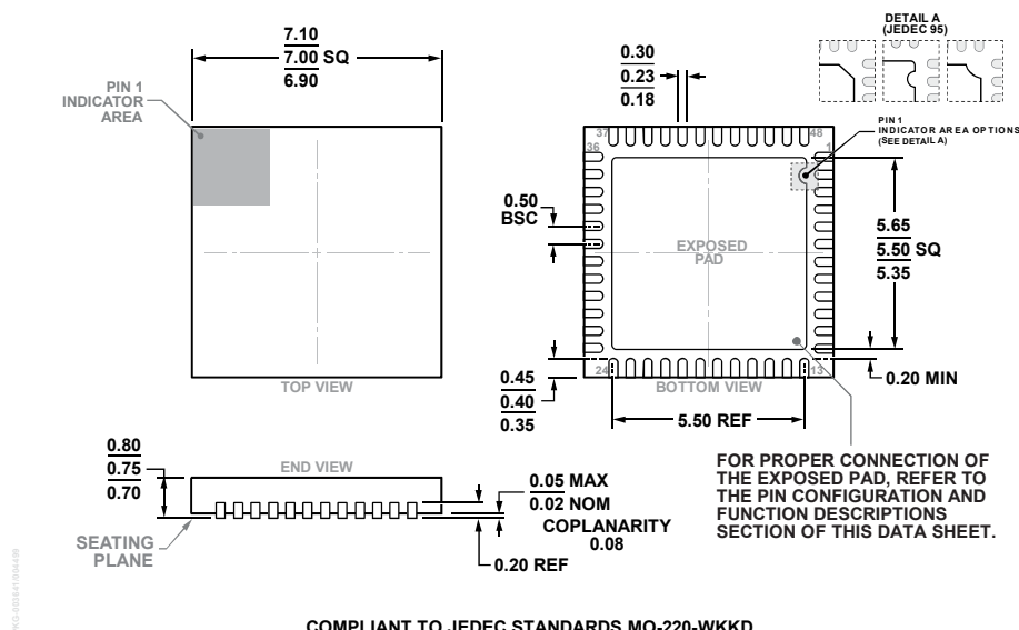
Figure 77. 48-Lead Lead Frame Chip Scale Package [LFCSP] 7 mm × 7 mm Body and 0.75 mm Package Height (CP-48-9)
