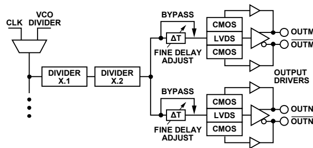
Figure 56. Fine Delay (OUT4 to OUT7)
