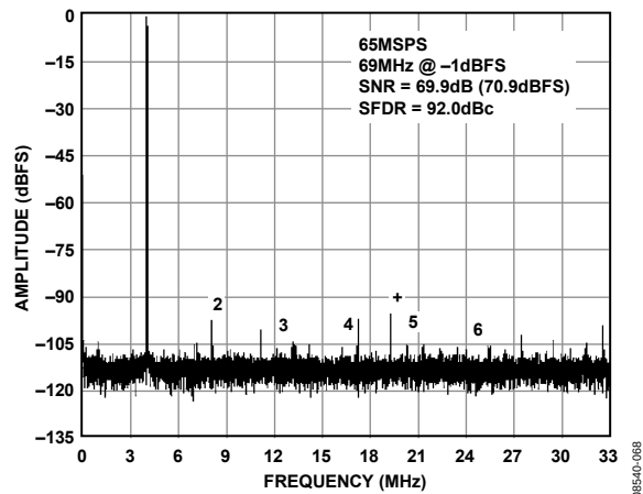
Figure 16. AD9629-65 Single-Tone FFT with f_{IN} = 69 MHz
