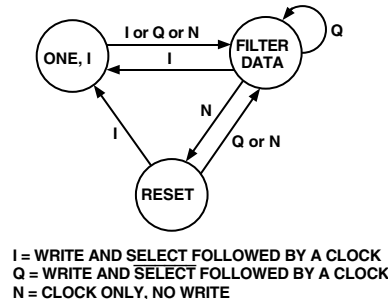
Figure 11. State Transition Diagram of AD9761 Digital Interface
