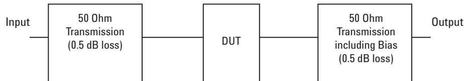
Block diagram of 900 MHz production test board used for V_d , Gain, P_{1dB} , OIP_3 , and NF measurements. Circuit losses have been de-embedded from actual measurements.
