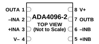
Figure 1. 8-Lead, MSOP (RM-8), ADA4096-2
