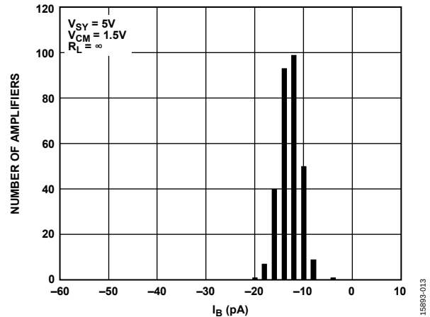
Figure 14. I_B Distribution, V_{SY} = 5 V
