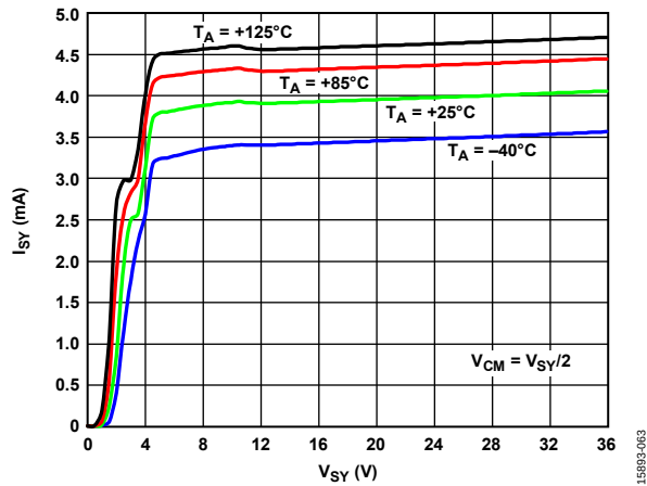
Figure 64. Supply Current ( I_{SV} ) vs. V_{SV} for Various Temperatures
