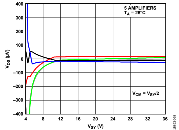
Figure 66. V_{OS} vs. V_{SV}
