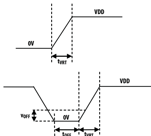
Figure 3. Power on Reset during power cycling
