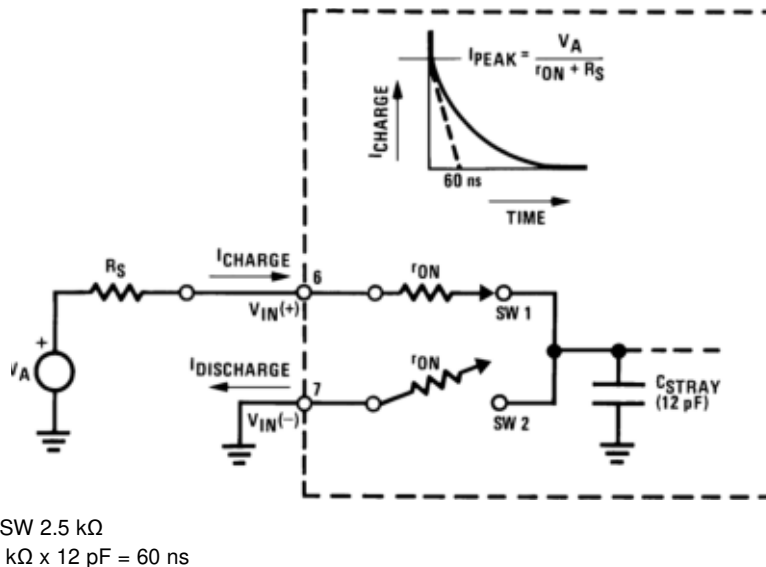
Figure 22. Analog Input Impedance
