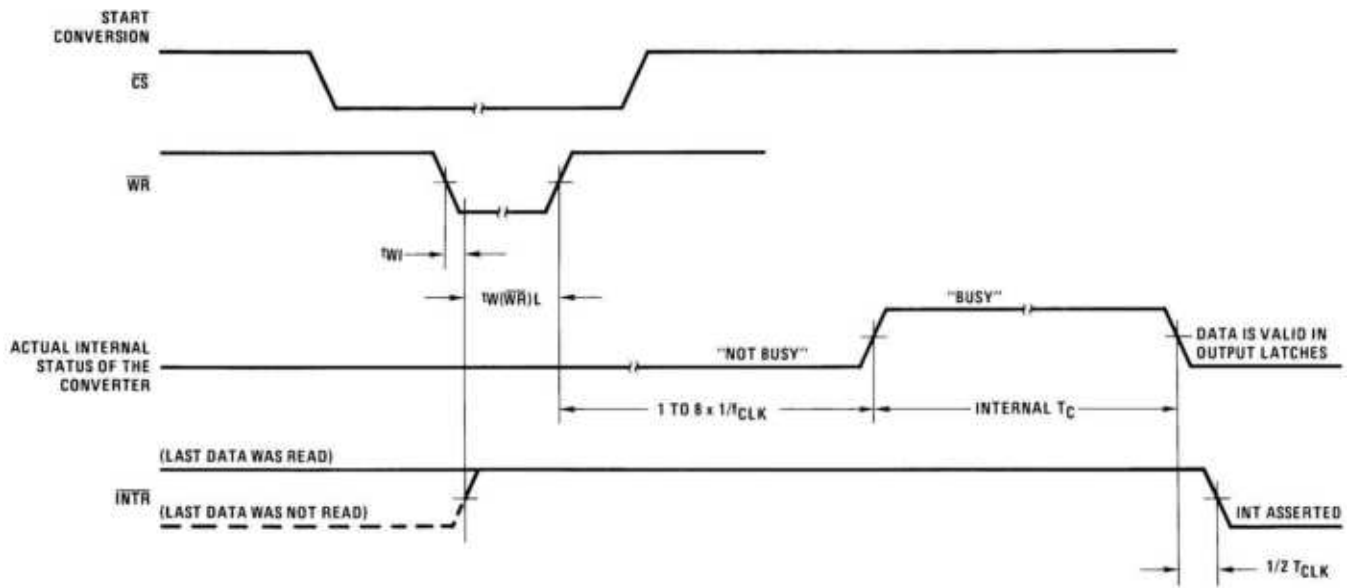
Figure 1. Start Conversion
