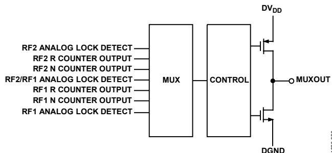
Figure 26. MUXOUT Circuit
