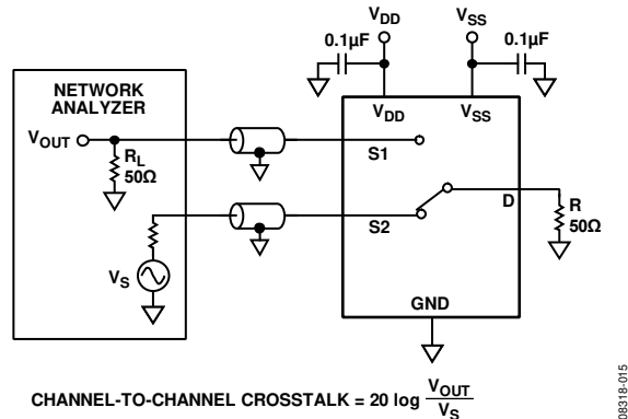
Figure 34. Channel-to-Channel Crosstalk
