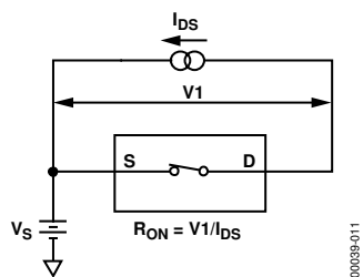
Figure 11. On Resistance
