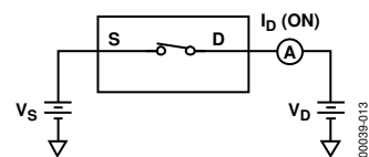
Figure 13. On Leakage
