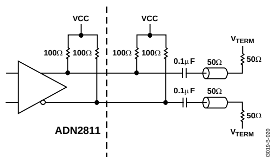
Figure 20. AC-Coupled Output Configuration
