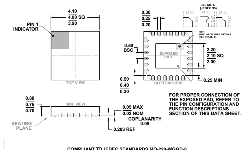
Figure 26. 24-Lead Lead Frame Chip Scale Package [LFCSP] 4 mm × 4 mm Body and 0.75 mm Package Height (CP-24-10) Dimensions shown in millimeters
