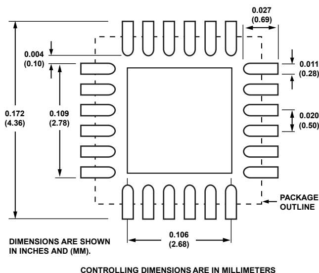
Figure 25. Suggested PCB Layout for the CP-24-10 Pad Landing
