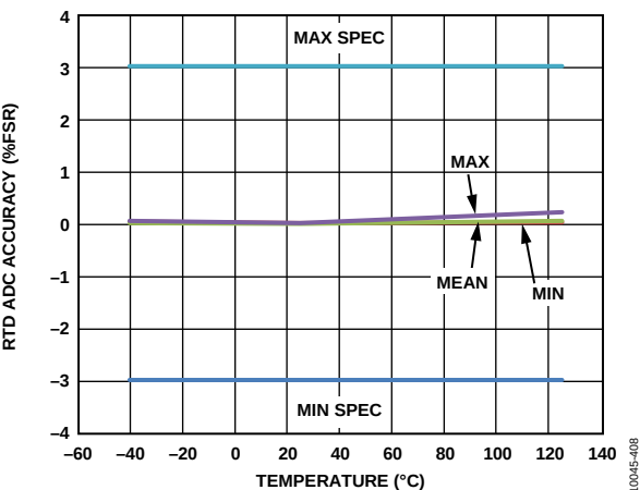
Figure 12. RTD ADC Accuracy vs. Temperature (from 10% to 90% of FSR)
