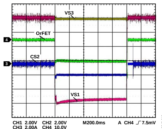
Figure 28. Internal Short Circuit (Yellow Is Bus Voltage; Red Is VS1 Voltage; Green Is OrFET Control Signal; Blue Is Load Current)
