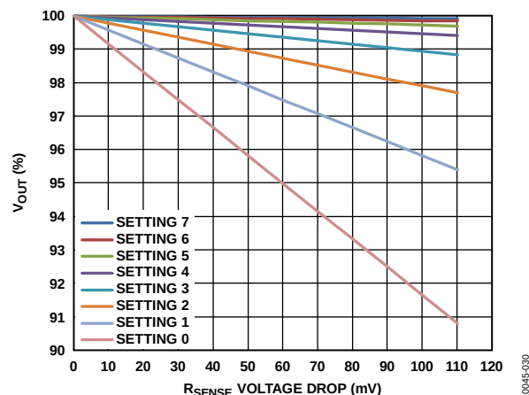
Figure 42. Load Line Settings with 120 mV CS2 Range
