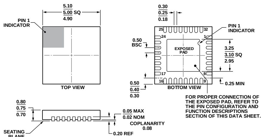
Figure 62. 32-Lead Lead Frame Chip Scale Package [LFCSP_WQ] 5 mm × 5 mm Body, Very Very Thin Quad (CP-32-7) Dimensions shown in millimeters
