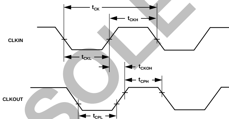
Figure 39. Clock Signals
