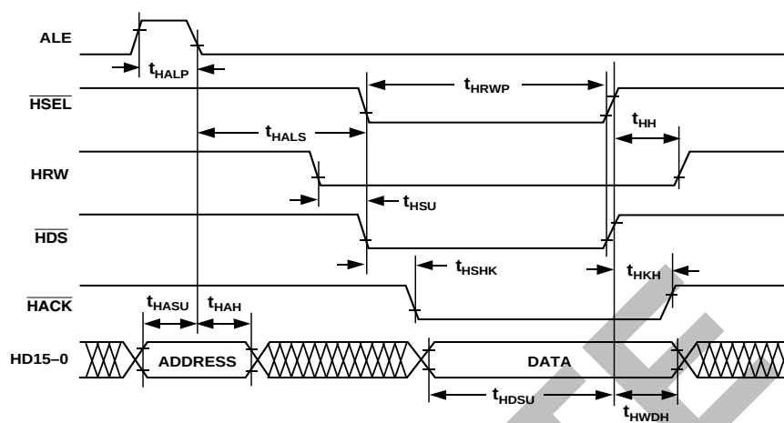
Host Write Cycle
