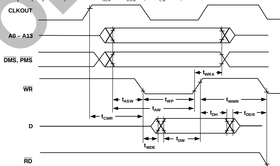
Figure 33. Memory Write
