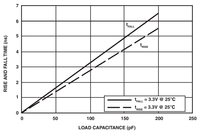
Figure 41. Driver Type C Typical Rise and Fall Times (10%–90%) vs. Load Capacitance (3.3V V_{DDEXT} )
