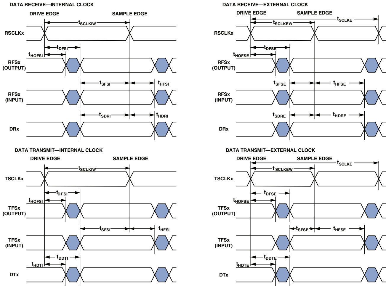
Figure 13. Serial Ports
