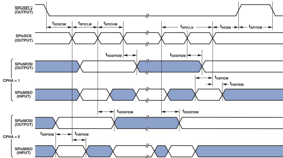
Figure 18. Serial Peripheral Interface (SPI) Port—Master Timing
