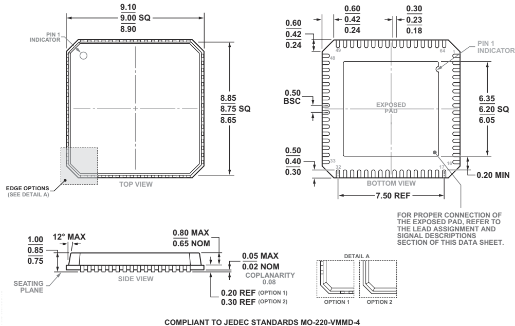
Figure 44. 64-Lead Lead Frame Chip Scale Package [LF CSP] 9 x 9 mm Body and 0.85 mm Package Height (CP-64-4) Dimensions shown in millimeters
