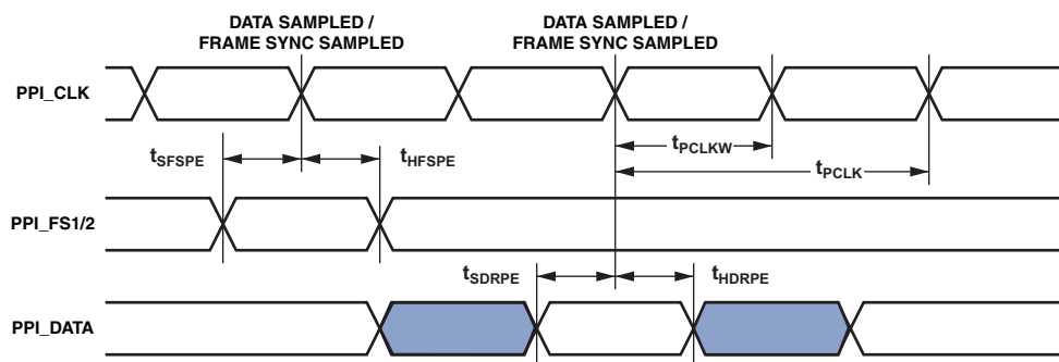
Figure 9. PPI GP Rx Mode with External Frame Sync Timing
