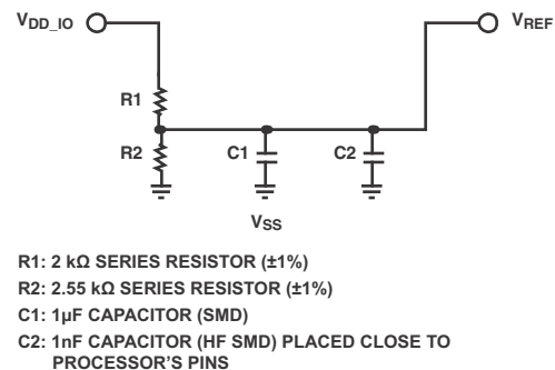
Figure 4. V_{\text{REF}} Filtering Scheme
