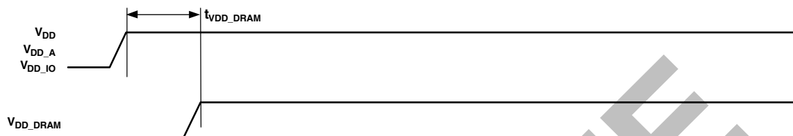
Figure 10. Power-Up Timing
