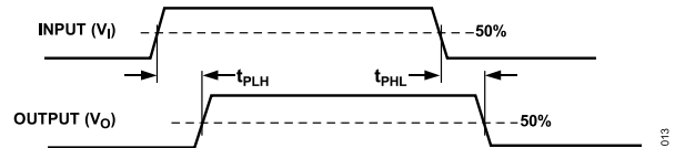
Figure 13. Propagation Delay Parameters
