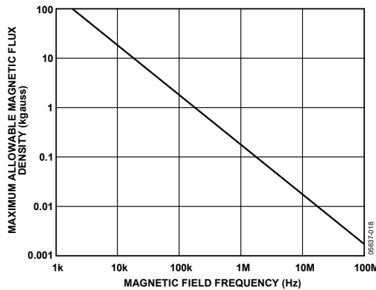
Figure 18. Maximum Allowable External Magnetic Field
