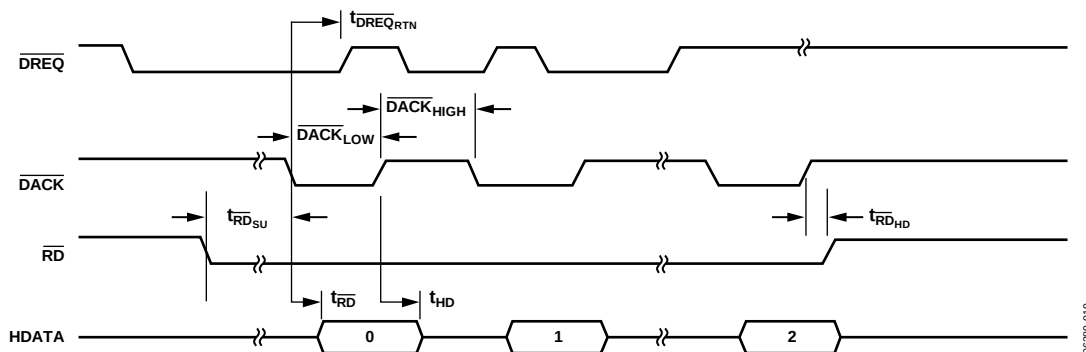
Figure 10. Single Read for DREQ/DACK DMA Mode for Assigned DMA Channel (EDMOD0/EDMOD1[14:11] Programmed to a Value of 0000)
