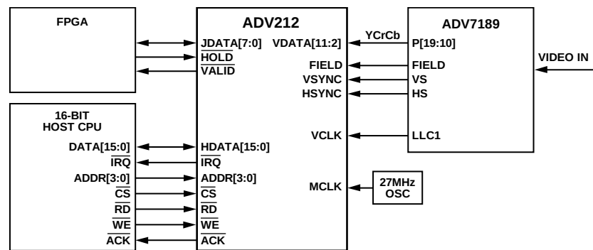
Figure 39. JDATA Application
