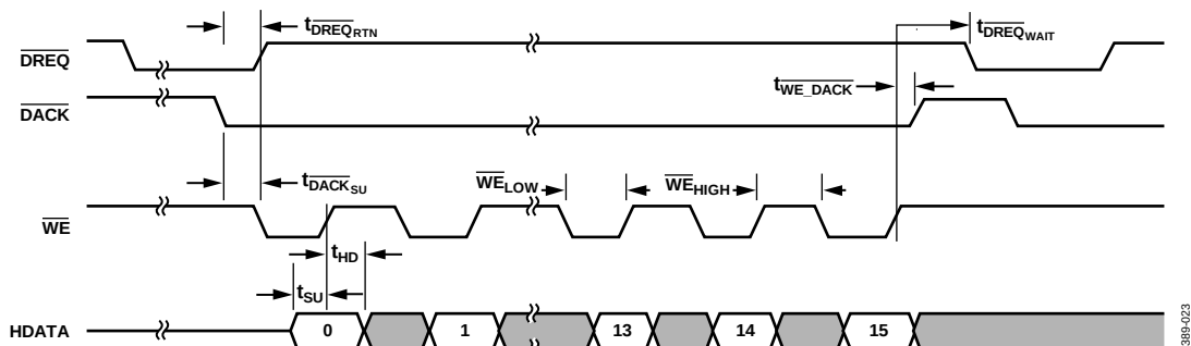
Figure 14. Burst Write Cycle for \overline{DREQ} /DMA Mode for Assigned DMA Channel (EDMOD0/EDMOD1[14:11] Programmed to a Value of 0000)
