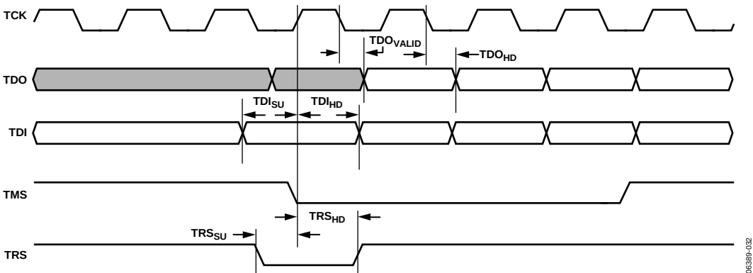
Figure 29. JTAG Timing
