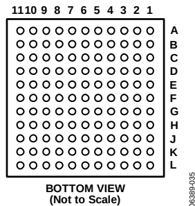
Figure 30. 121-Ball Pin Configuration
