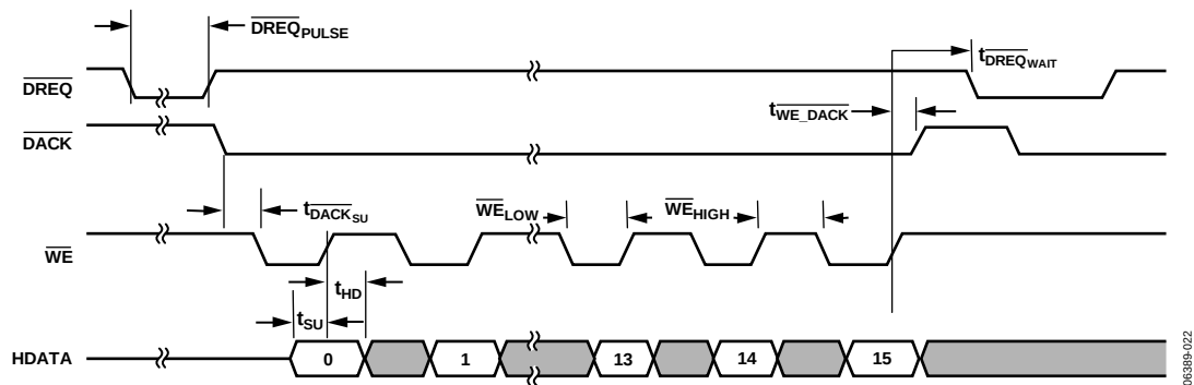
Figure 13. Burst Write Cycle for \overline{DREQ} /DMA Mode for Assigned DMA Channel (EDMOD0/EDMOD1[14:1] Not Programmed to a Value of 0000)
