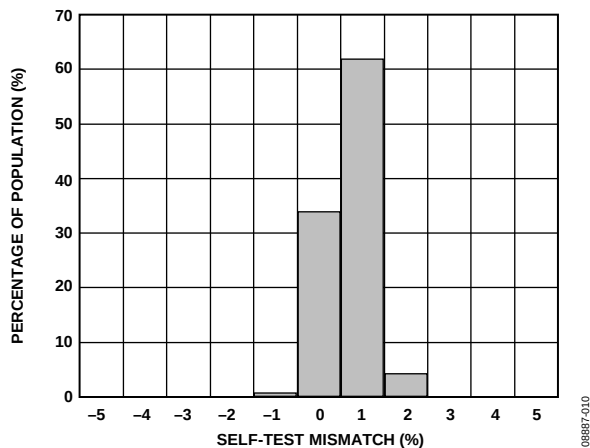
Figure 10. Self-Test Mismatch at 25°C ( V_{RATIO} = 5\text{ V} )
