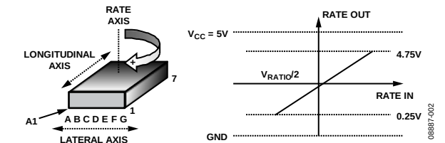
Figure 2. RATEOUT Signal Increases with Clockwise Rotation
