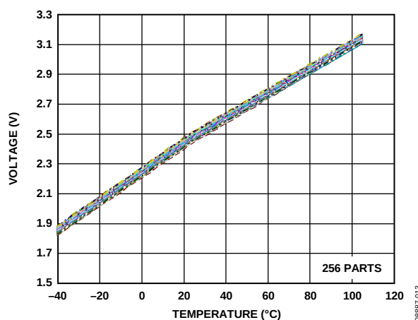
Figure 14. V_{TEMP} Output over Temperature ( V_{RATIO} = 5\text{ V} )
