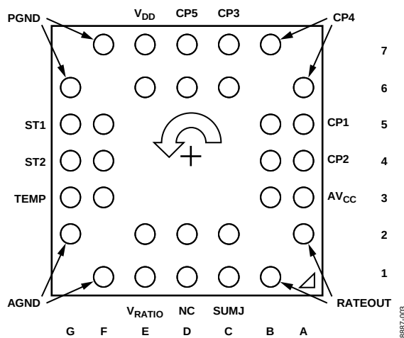
Figure 3. Pin Configuration
