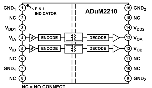
Figure 1. ADuM2210
