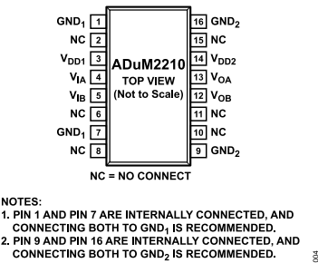
Figure 4. ADuM2210 Pin Configuration
