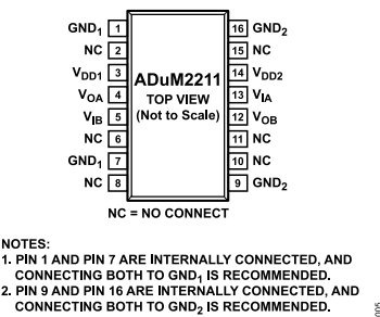
Figure 5. ADuM2211 Pin Configuration
