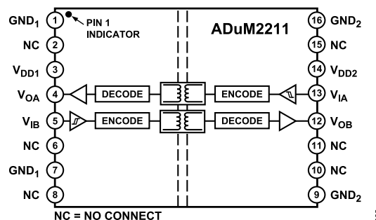
Figure 2. ADuM2211
