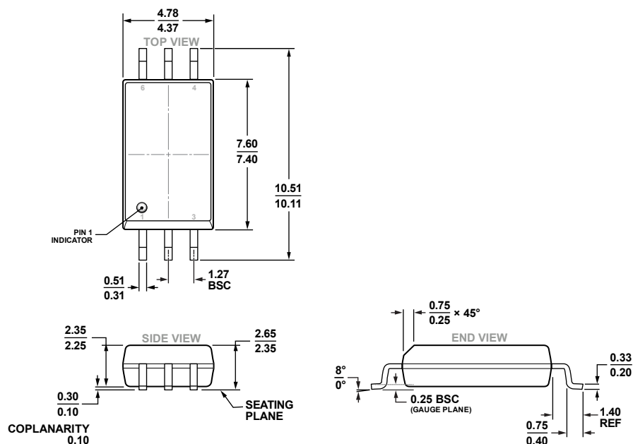
Figure 27. 6-Lead Standard Small Outline Package, with Increased Creepage [SOIC_IC] Wide Body (RI-6-1)
