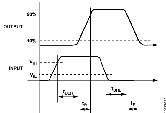
Figure 22. Propagation Delay Parameters
