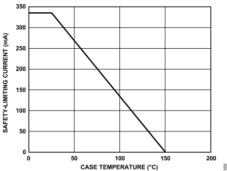
Figure 5. Thermal Derating Curve, Dependence of Safety-Limiting Values on Case Temperature per DIN EN IEC 60747-17 (VDE 0884-17)
