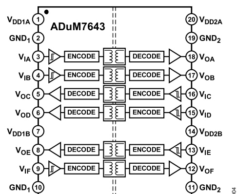
Figure 4. ADuM7643
