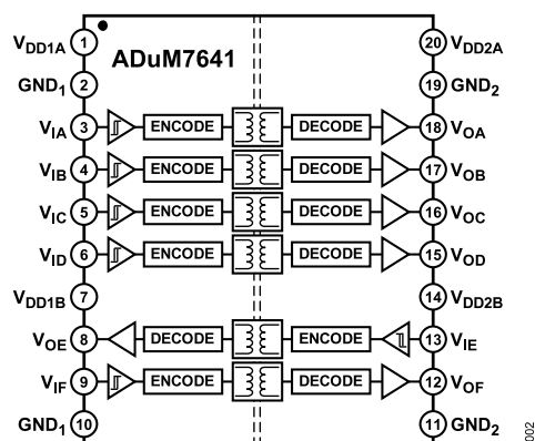
Figure 2. ADuM7641
