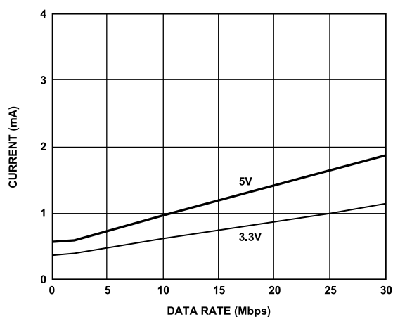
Figure 11. Typical Supply Current per Output Channel vs. Data Rate for 5 V and 3.3 V Operation (No Output Load)
