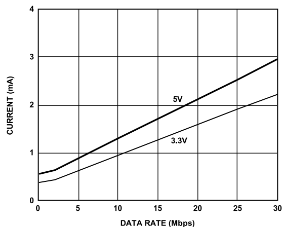
Figure 12. Typical Supply Current per Output Channel vs. Data Rate for 5 V and 3.3 V Operation (15 pF Output Load)
