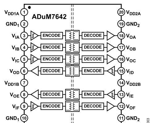
Figure 3. ADuM7642
