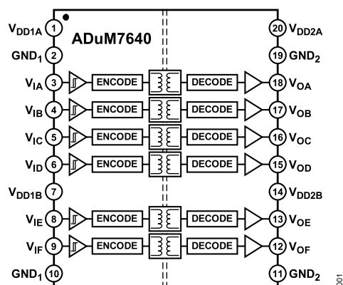
Figure 1. ADuM7640
