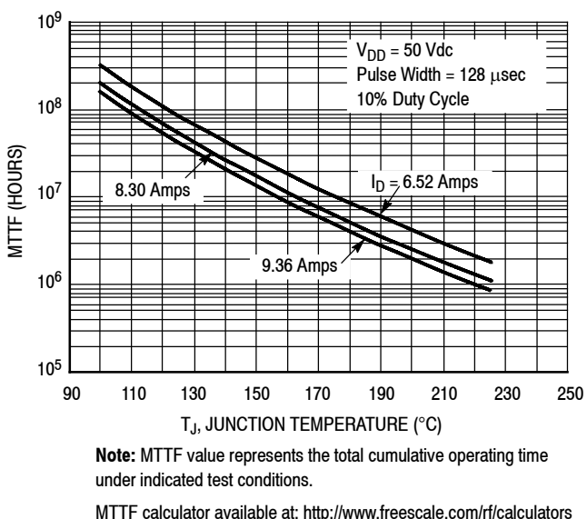
Figure 4. MTTF versus Junction Temperature - Pulse
