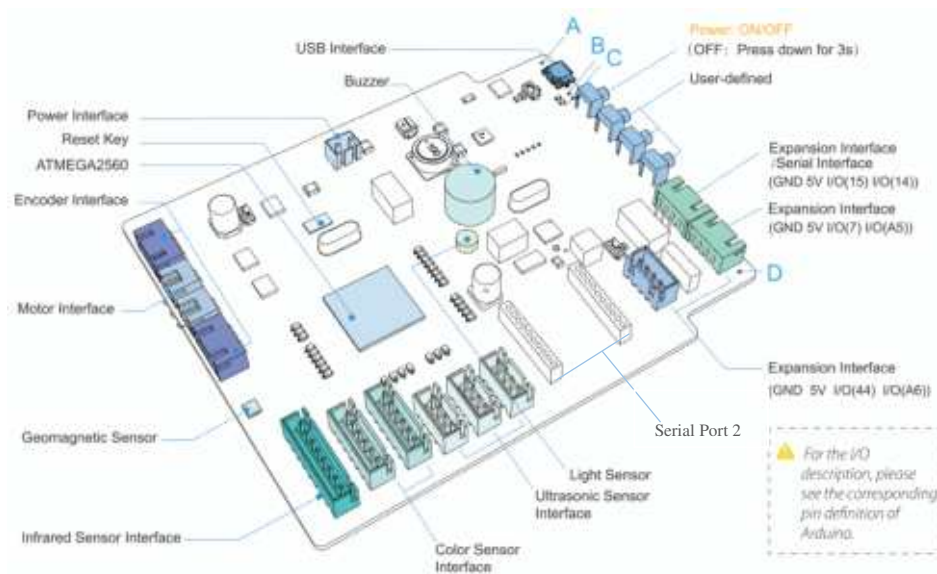
Figure 3.1 AI-Starter control board description
