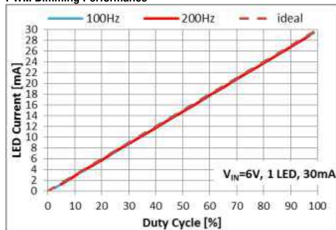
Figure 8 PWM Dimming 30mA vs. Duty Cycle
