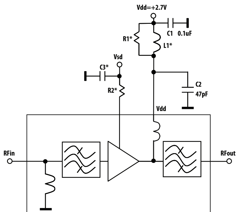
Figure 2. Application Circuit
