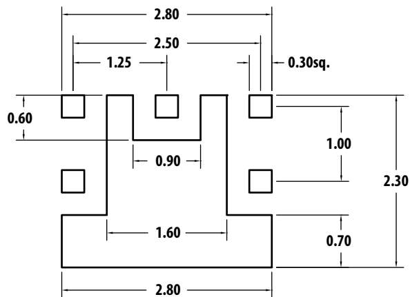
Land Pattern
