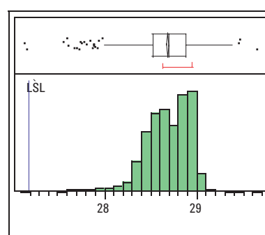
P-1dB at 18 GHz
