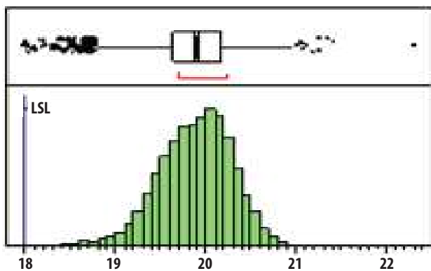
Figure C. Gain @ 40GHz, Nominal = 20, LSL = 18
