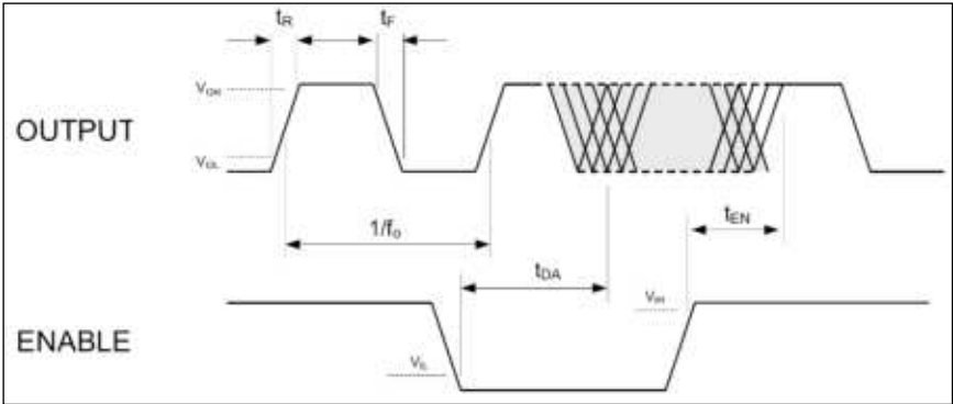
Output Waveform
