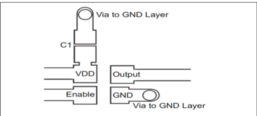
Recommended Board Layout
