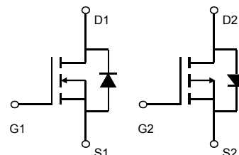
N-channel
