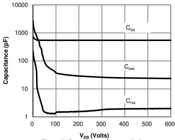
Figure 9: Capacitance Characteristics
