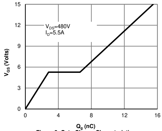
Figure 8: Gate-Charge Characteristics
