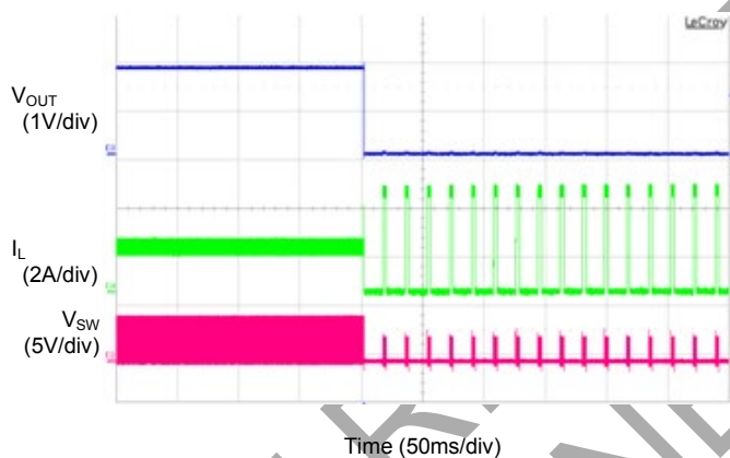
Short Current Protection ( I_{OUT}=2\text{A} )
