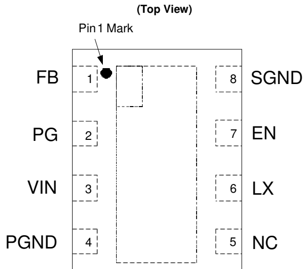
U-DFN2020-8 (Type E)
